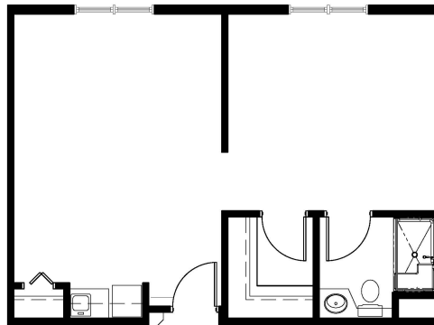
ONE BEDROOM II 600 SQ FT
